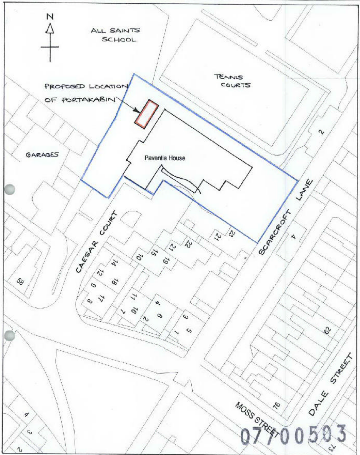
YORK FAMILY HOUSING CAESAR COURT, YORK LOCATION PLAN 1:500
